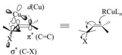
Figure 1. Proposed interaction of the frontier orbitals previous to the S N 2' reaction.
